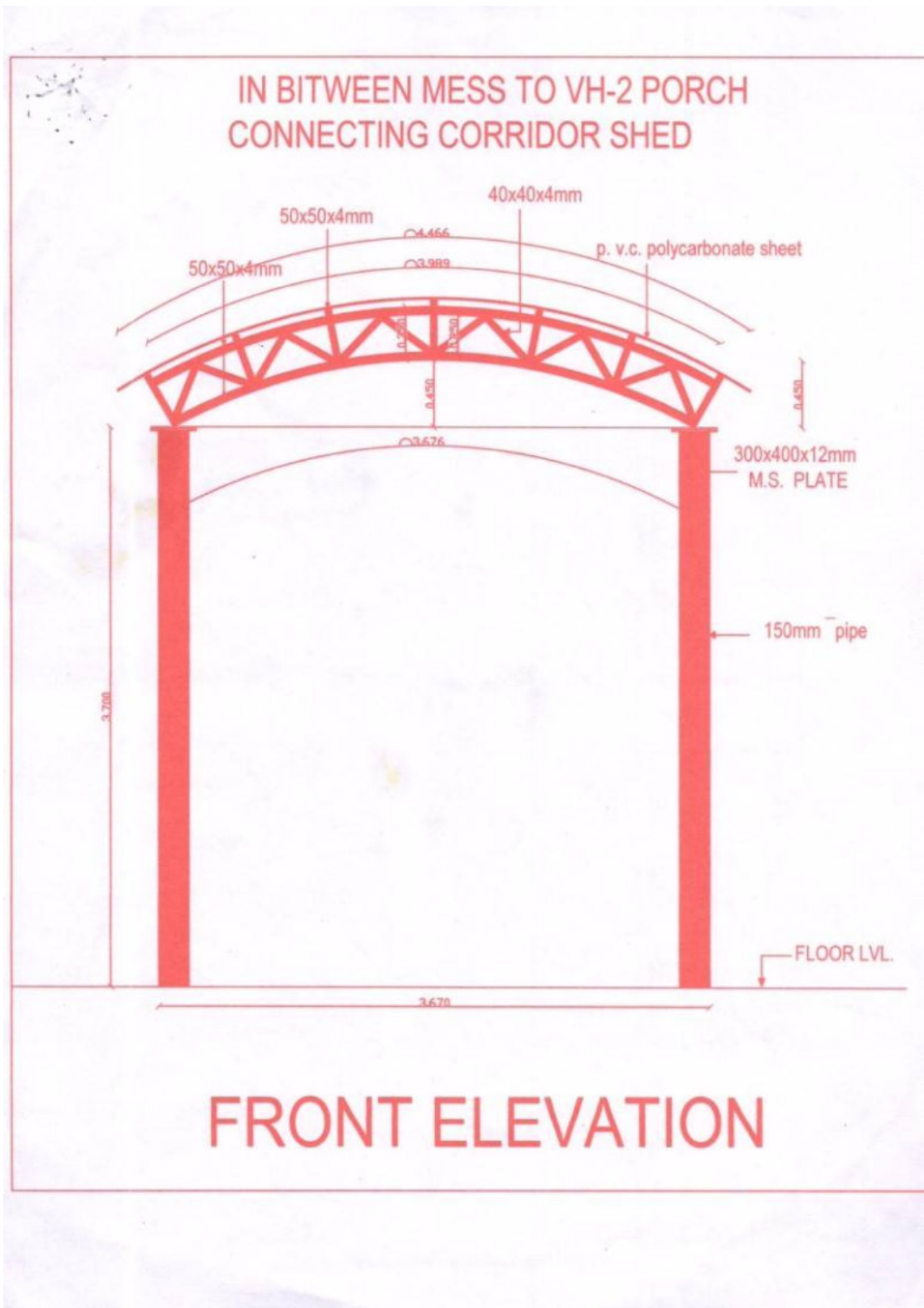
Figure 3: Front elevation drawing of the shed to be constructed
